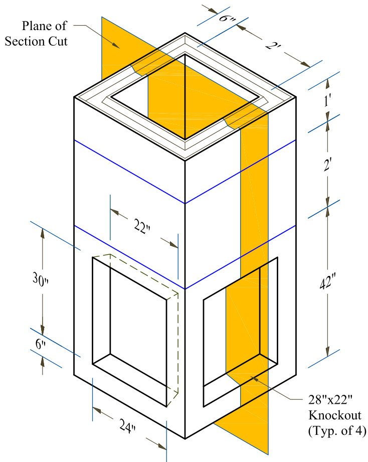
Isometric View
