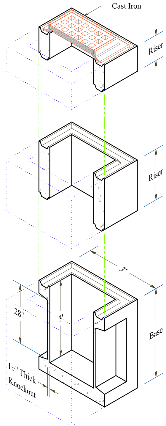
Exploded Section
