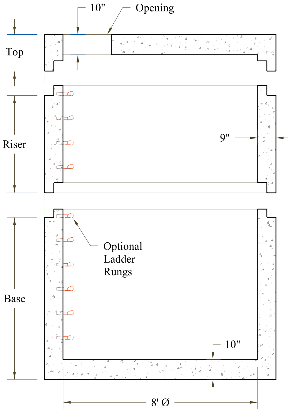
Section View
