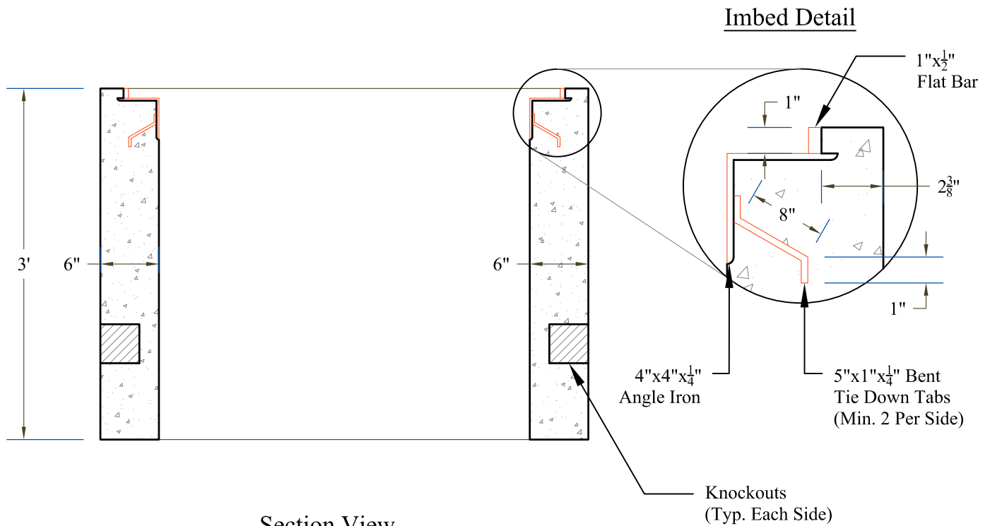
Section View
