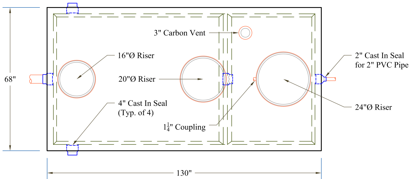
Plan View
