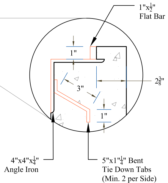
Imbed Detail
