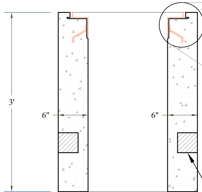
Section View
