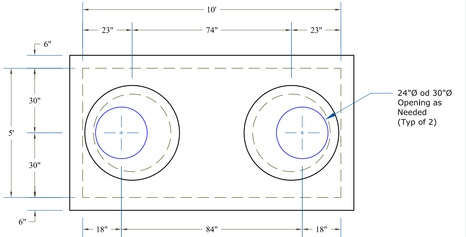
Plan View
