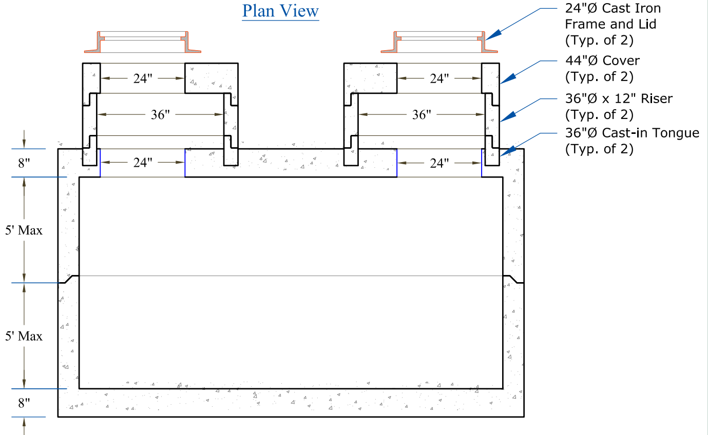
Section View
