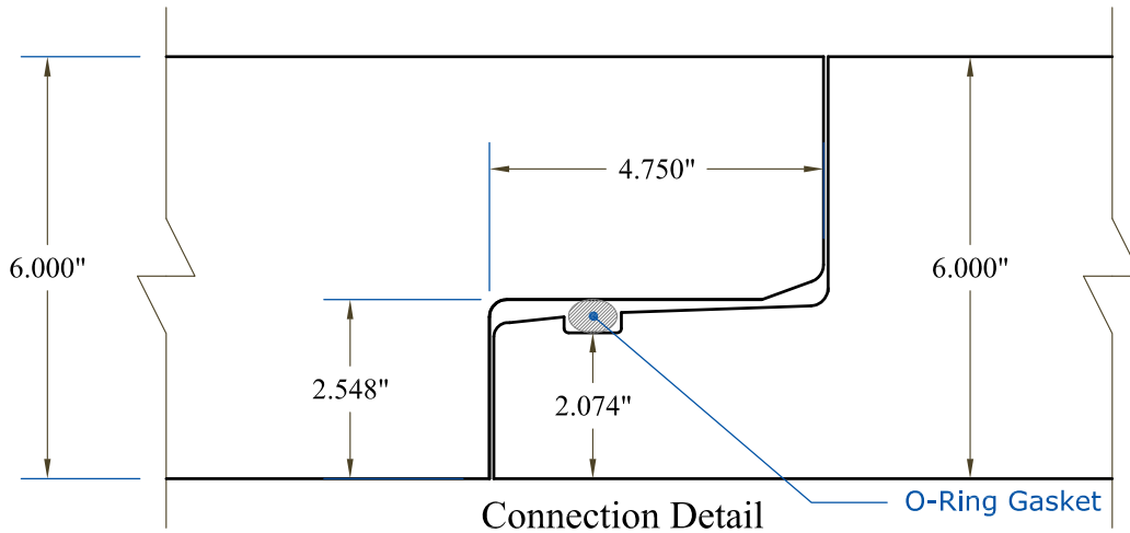
Section View
