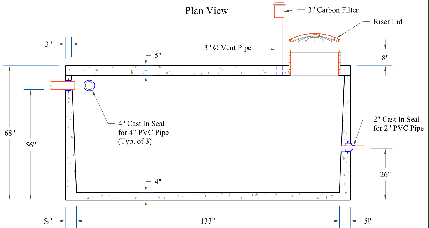
Section View
