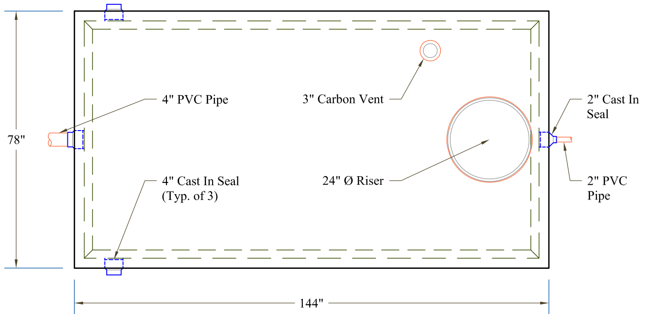
Plan View
