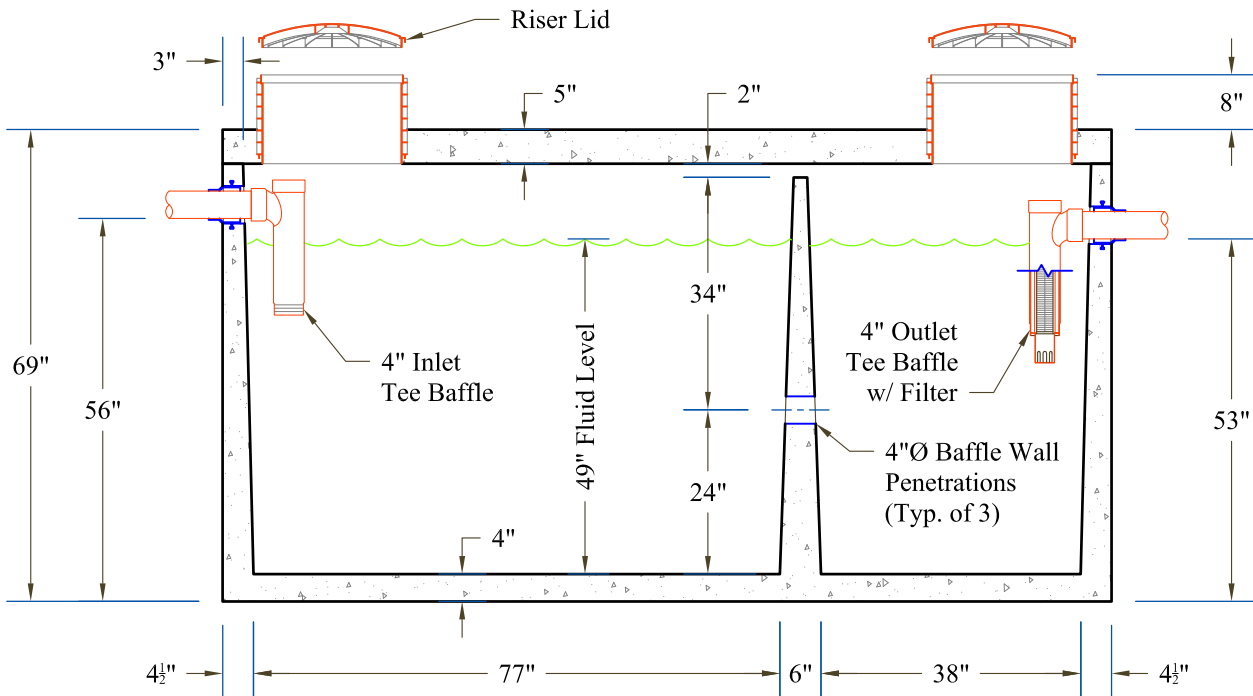
Section View
