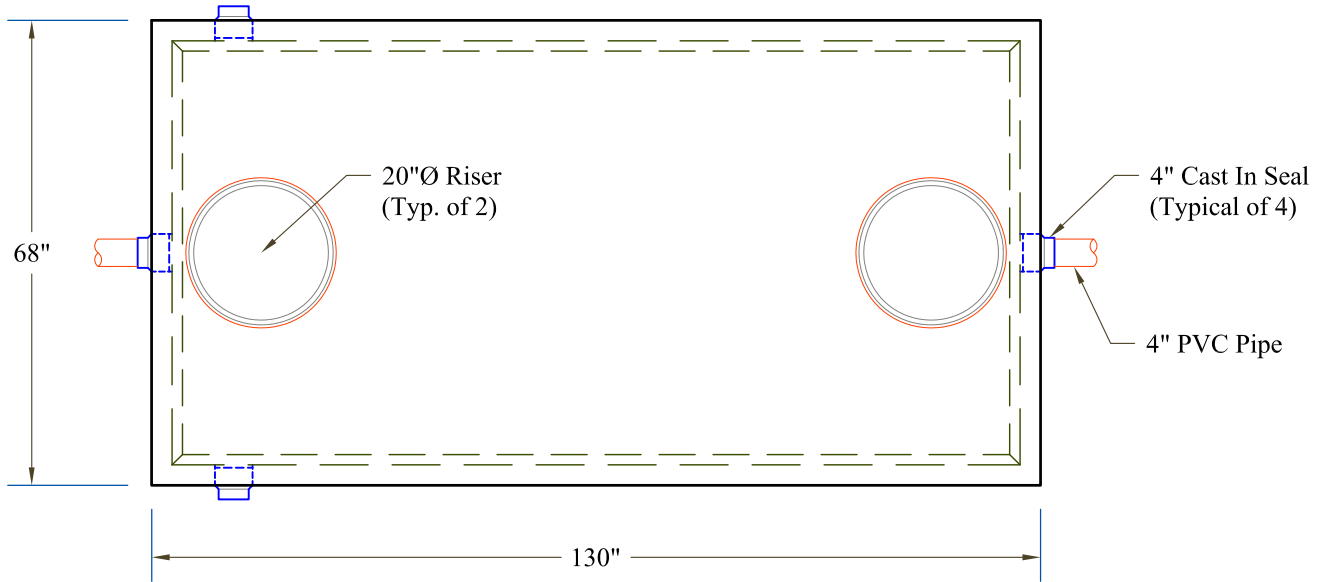
Plan View
