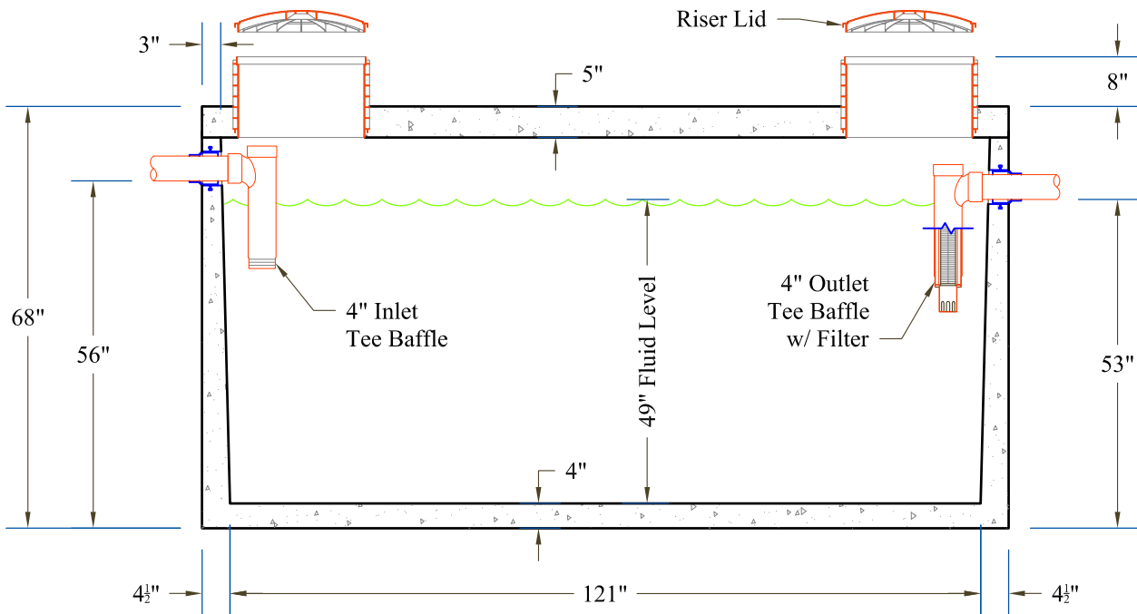
Section View
