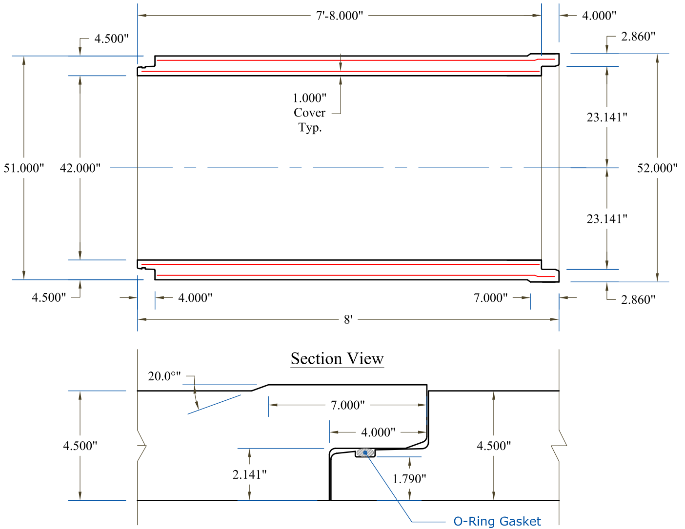
Connection Detail
