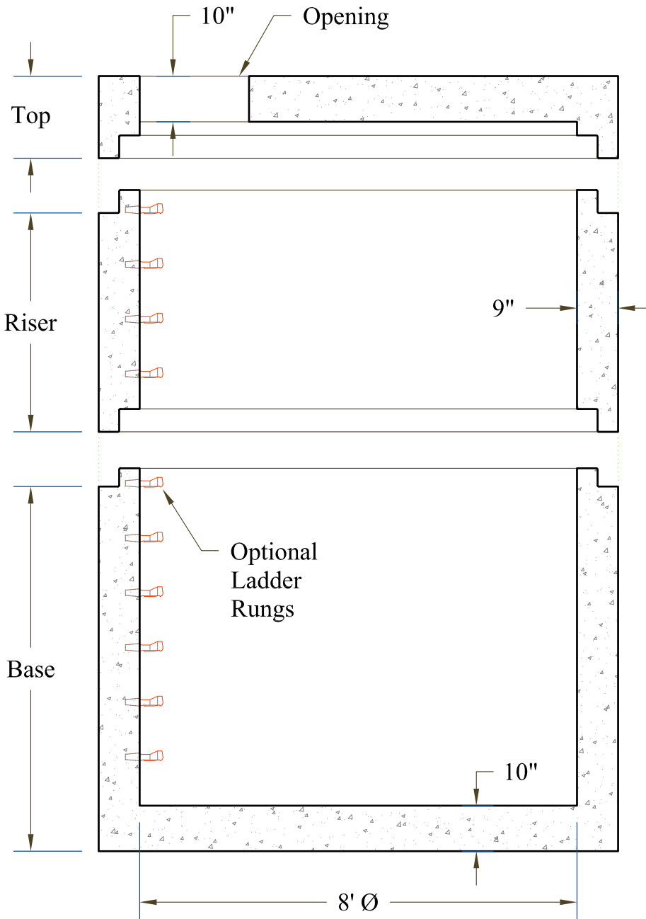
Section View
