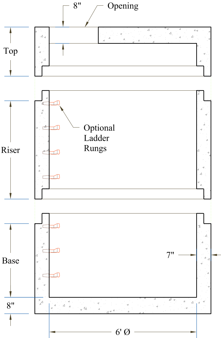
Section View
