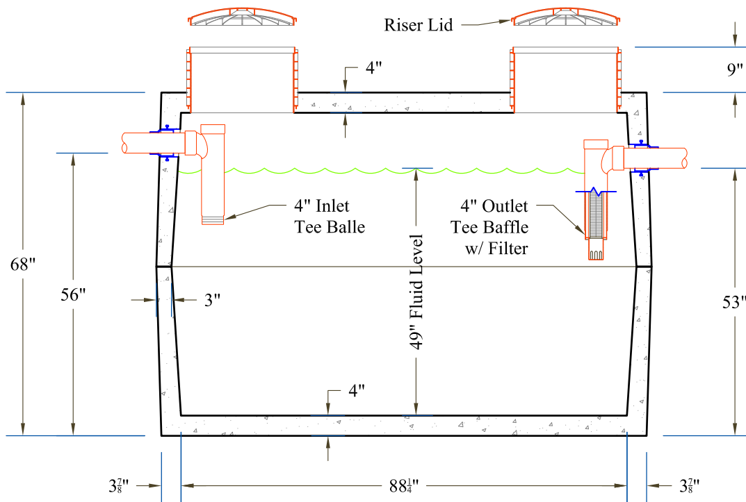
Section View
