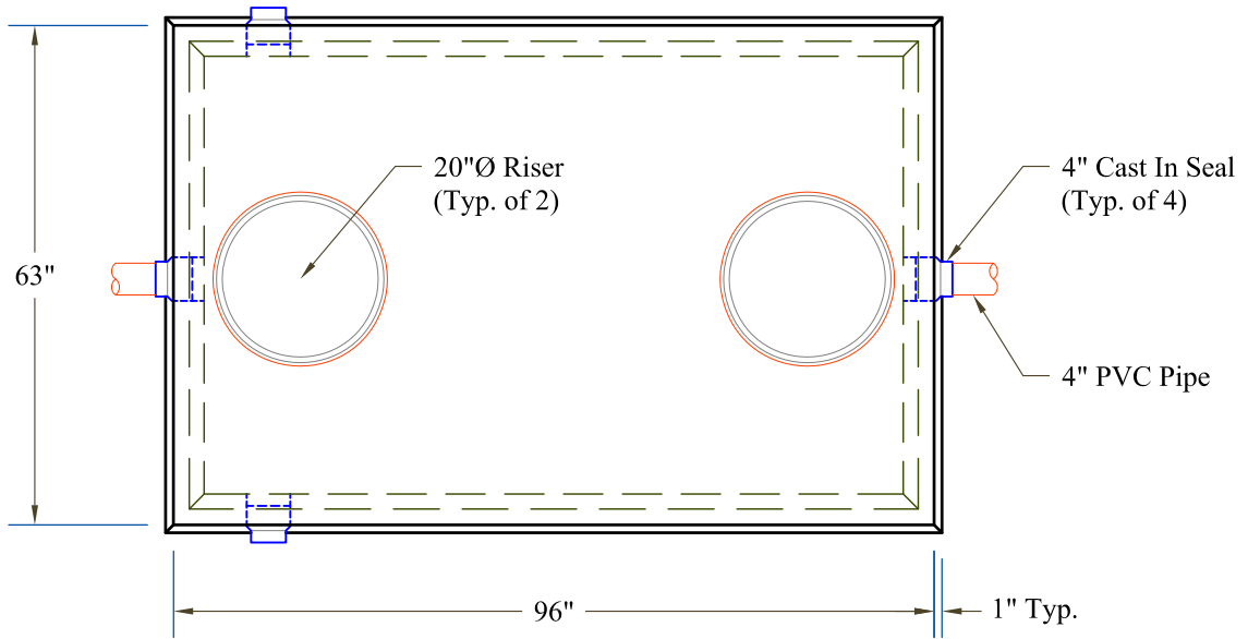
Plan View
