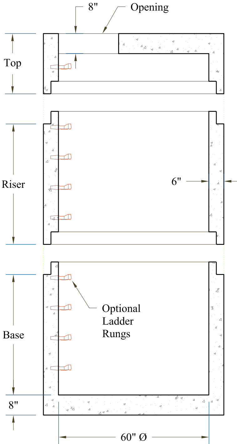
Section View
