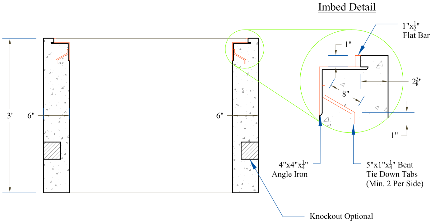
Section View
