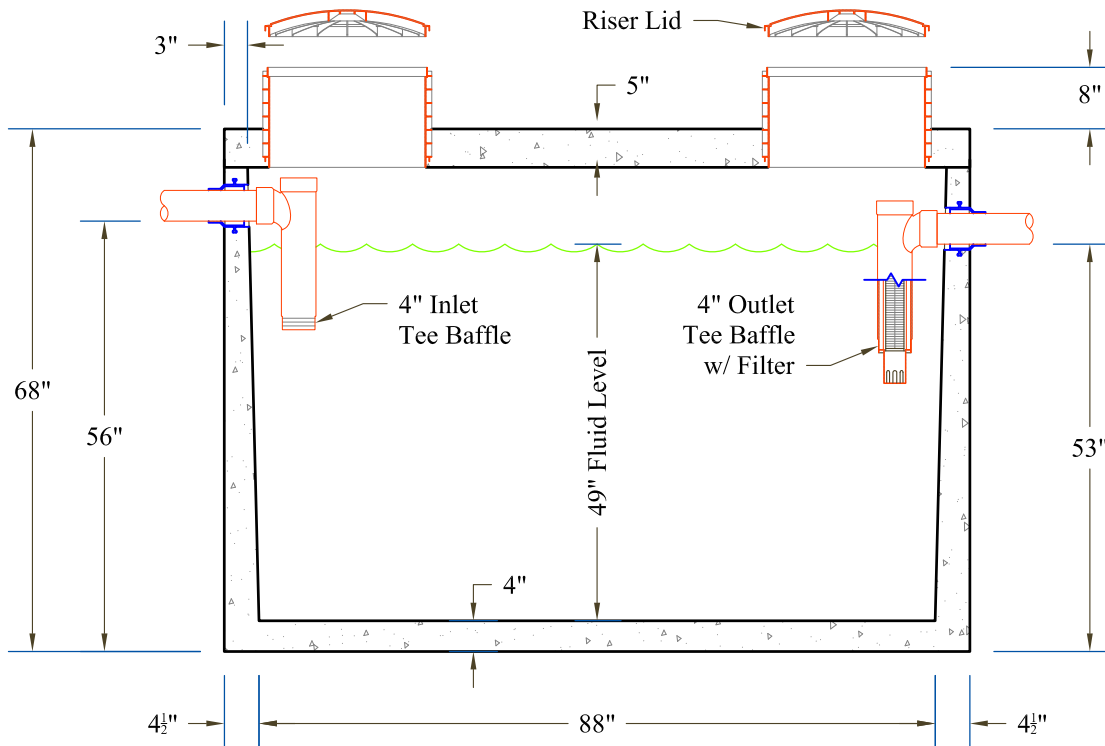
Section View
