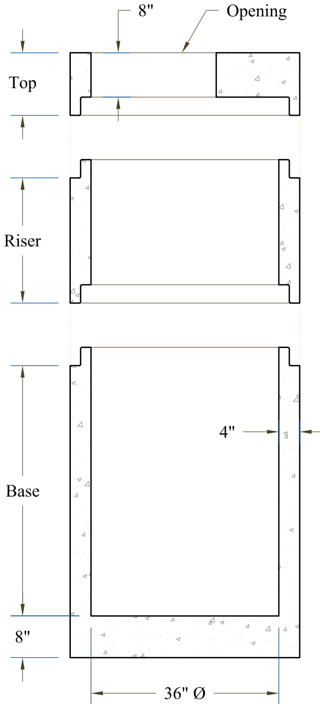
Section View
