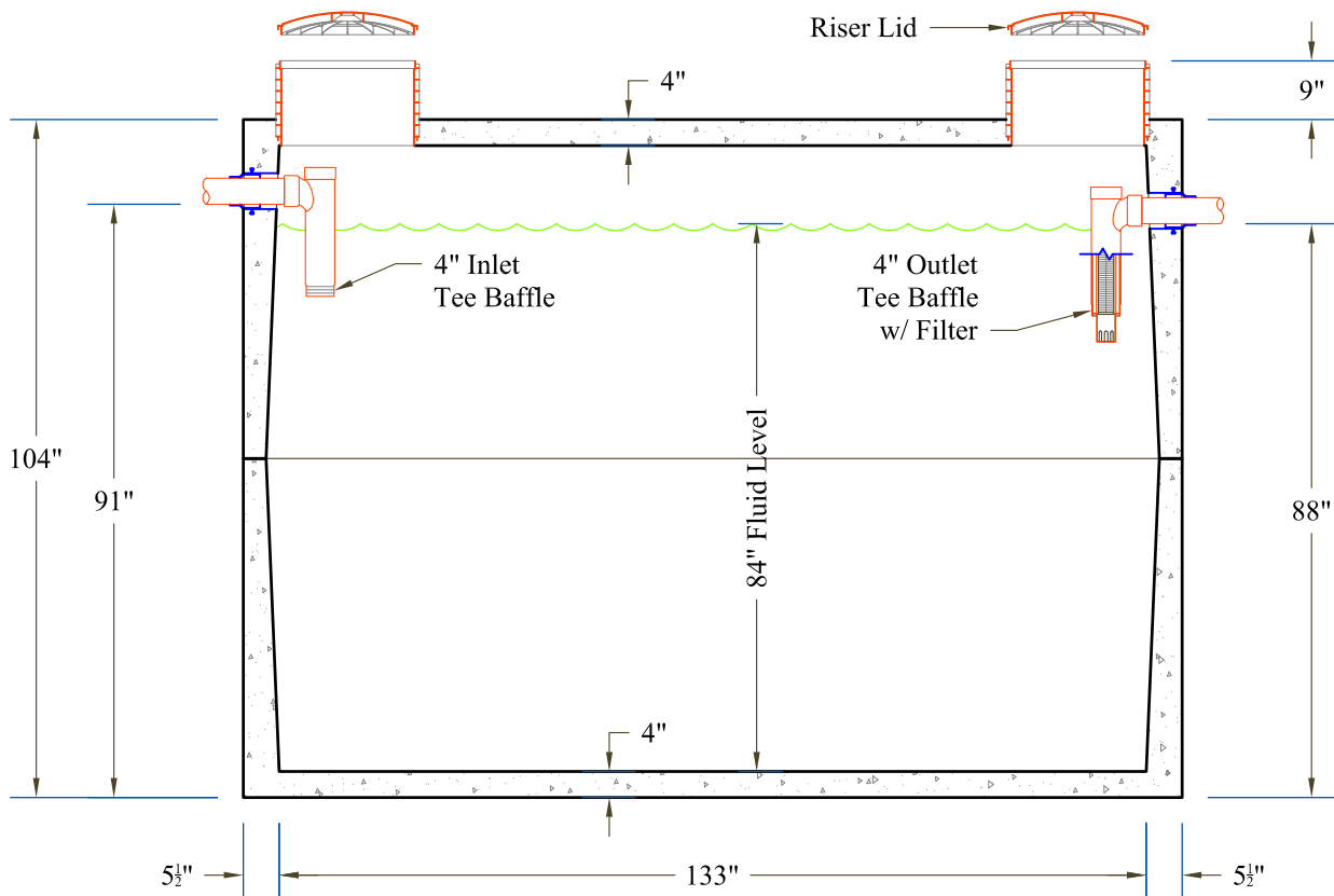
Section View
