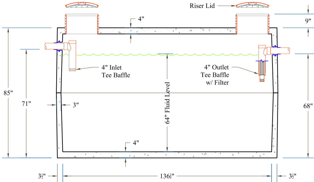
Section View
