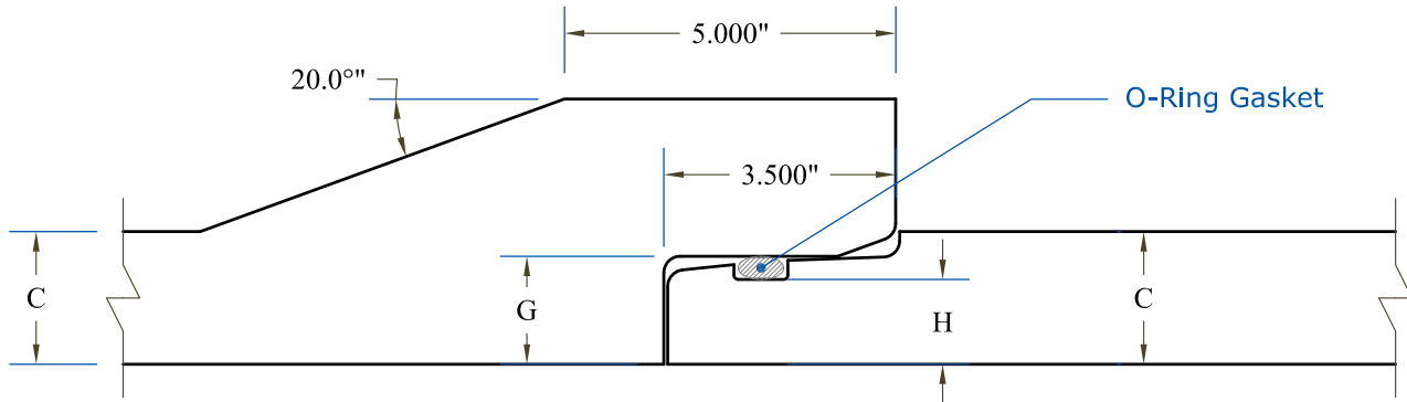
Connection Detail
