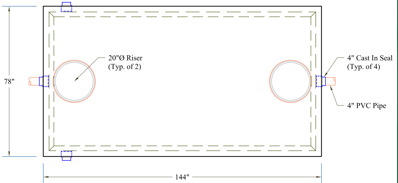
Plan View
