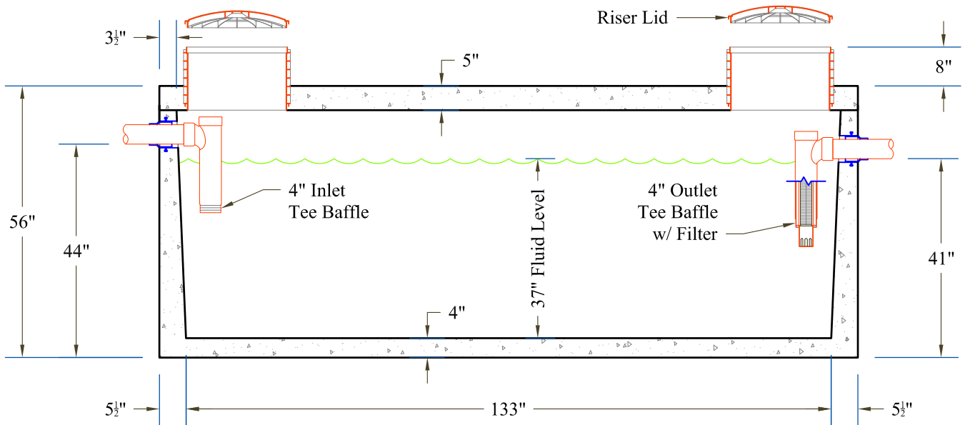
Section View
