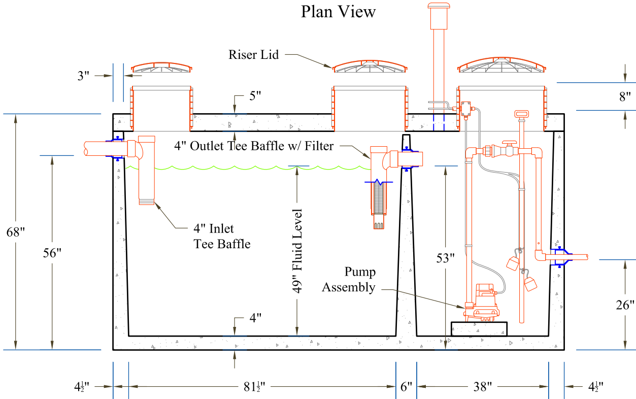
Section View
