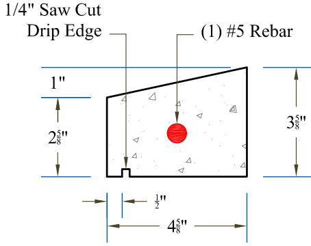
Section View
