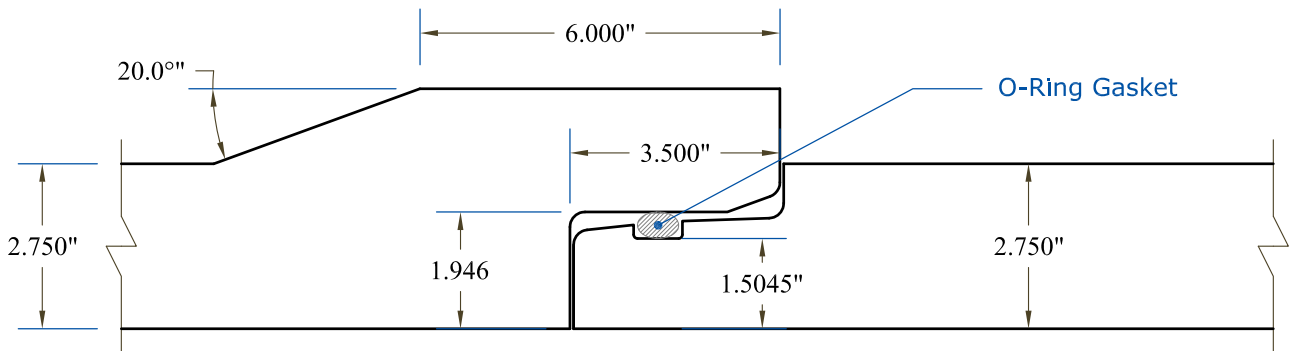
Connection Detail
