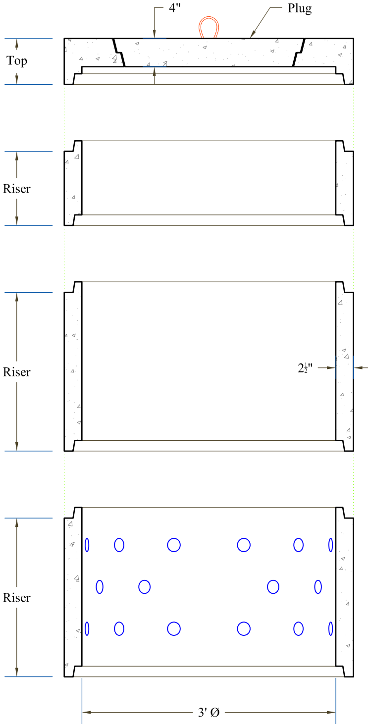
Section View
