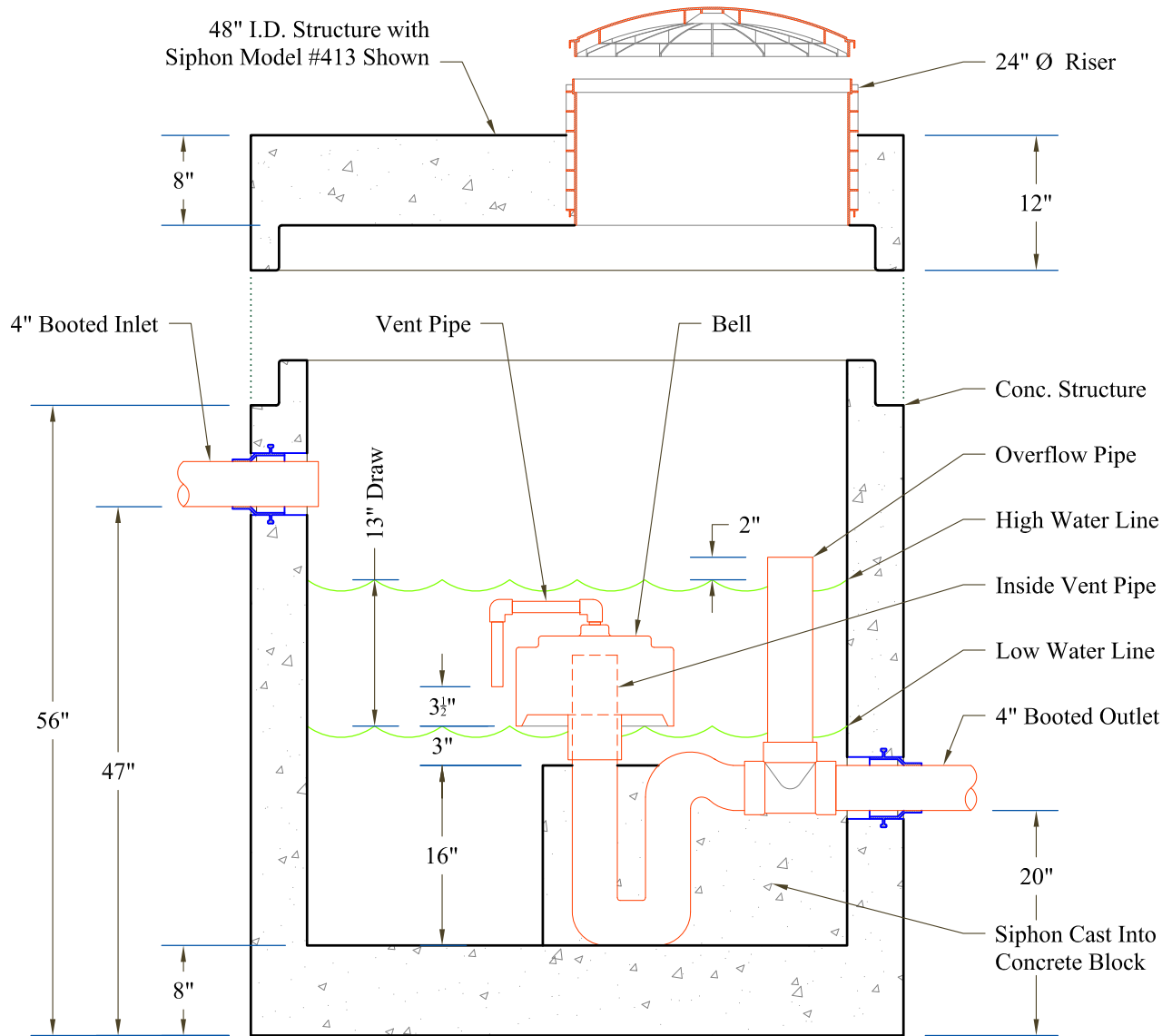
Section View
